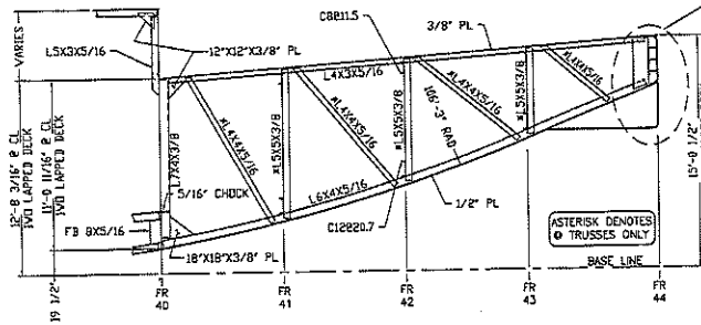
LONG'L BOW RAKE TRUSS PORT SIDE LOOKING OUTBD
