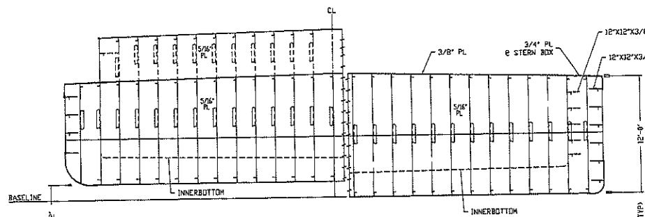
PARTIAL SECTION @ FWD COLLISION BHD (LOOKING AFT)
