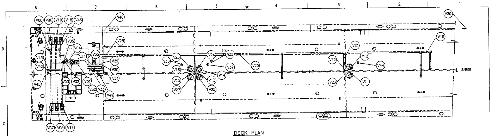
DECK PLAN
