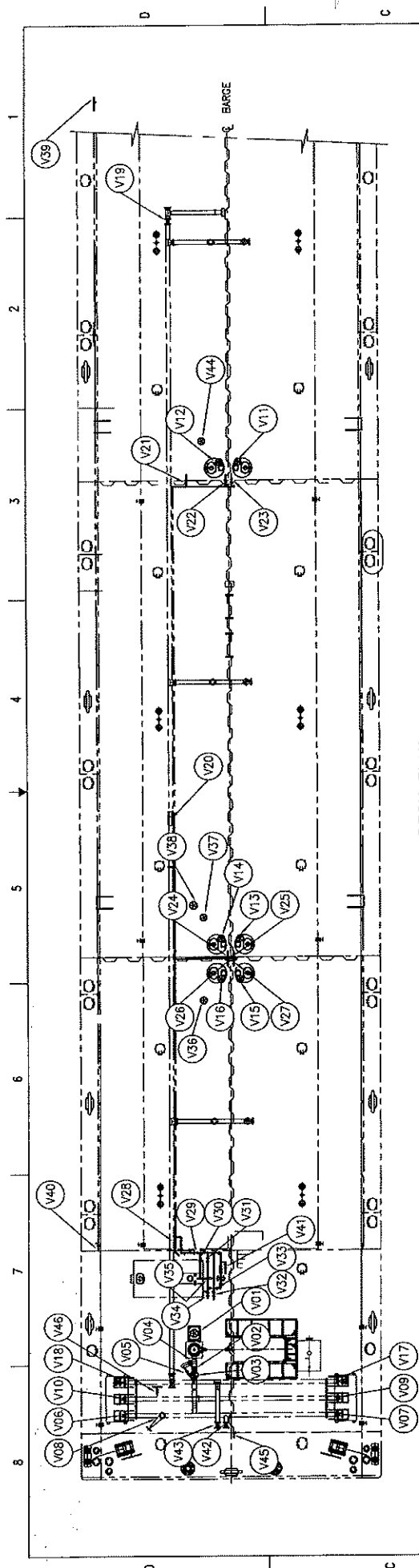
DECK PLAN
