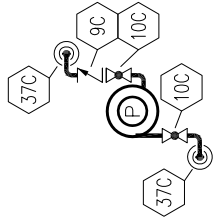
DEEPWELL CAN PUMP DETAIL
